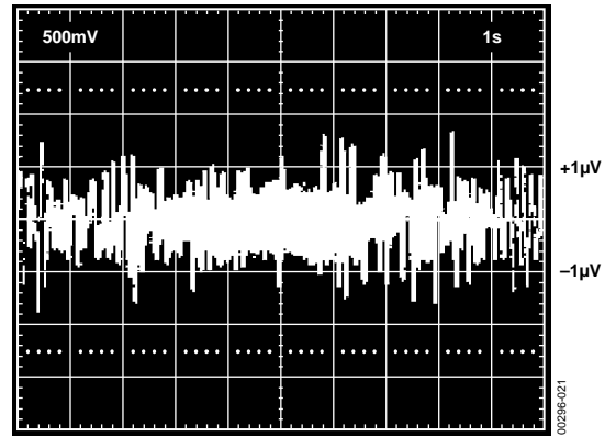
BANDWIDTH (0.1Hz TO 10Hz) TA = 25°C, VS = ±15V
